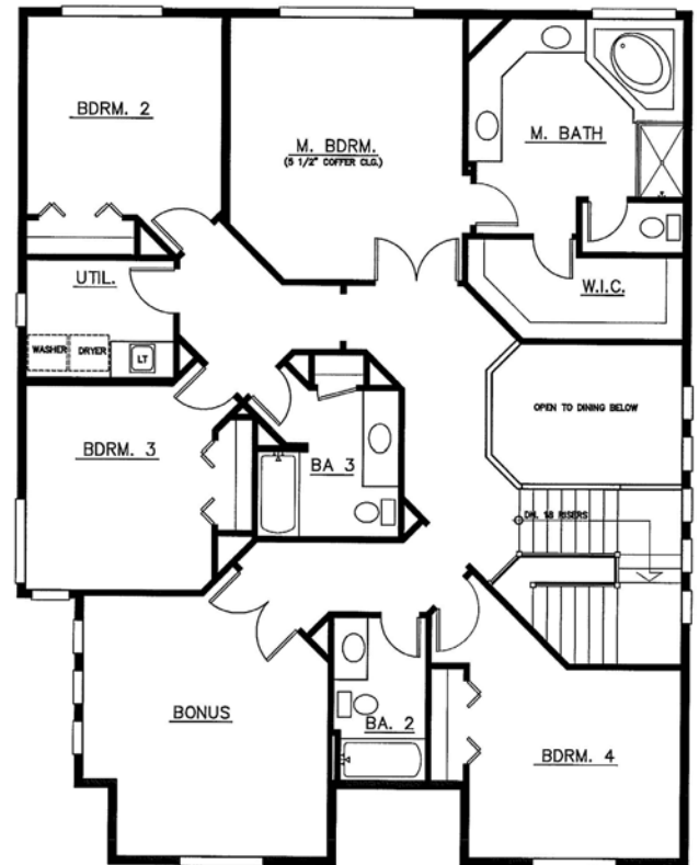
Upper Floor
